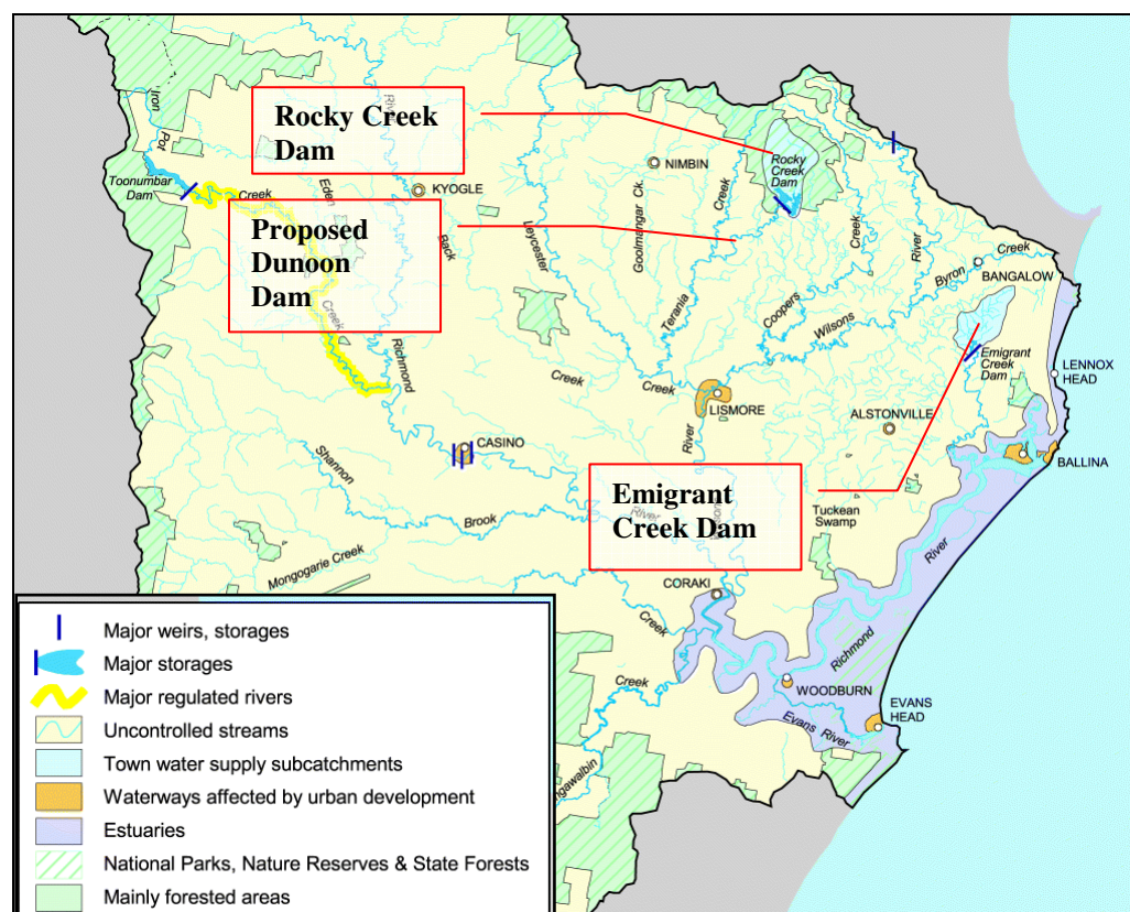
Figure 1 Richmond River Catchment including Rous Water Catchment Areas
